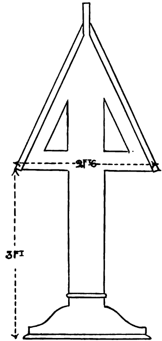
FIG. 30.—Double Newspaper Stand showing Dimensions (Section 163).
